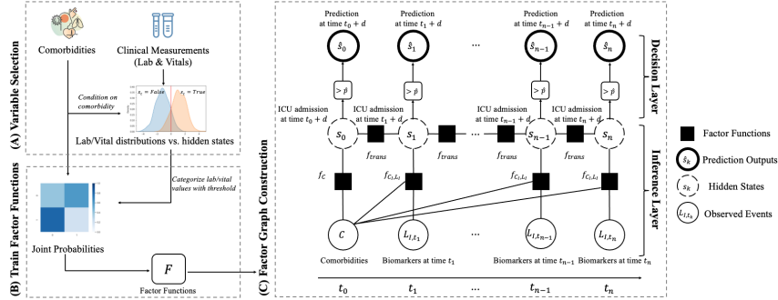
Fig. 1.1 Approach Overview. (A) For each comorbidity, lab/vital distributions are plotted with respect to the label (ICU/No ICU). The thresholds that best separate the distribution are computed. (B) Thresholds are used to categorize the lab/vital values and calculate the joint probabilities to construct FFs. (C) FGs are constructed by connecting FFs with observed events and hidden states. Predictions are made based on a threshold for the hidden state probabilities learned from the training data. C = \{c_1, \dots, c_6\} is a set of comorbidity nodes; L_{I,t_k} = \bigcup_{i \in I} L_{i,t_k} is a union of the sets of predictive biomarkers L_i for the patient's comorbidities c_i \in C_I ; f_C = \{f_{c_1}, \dots, f_{c_6}\} is a set of Comorbidity FFs; f_{C,I,L_I} = \bigcup_{i \in I} (\bigcup_{l_j \in L_i} f_{c_i,l_j}) is a union of the Bio FFs.
